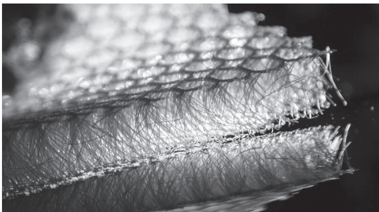
Figure 12. 3D spacer fabric [38].
